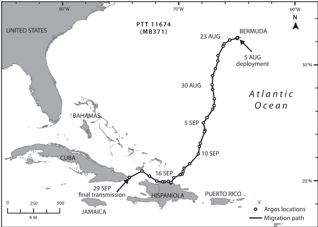
Fig. 12. Satellite transmission history of a large subadult (78.6 cm SCL min ) Chelonia mydas from Bermuda. Argos locations displayed are the highest location class per day, selected from the hybrid output of the Douglas Argos filter algorithm. This output includes points passing the minimum redundant distance filter supplemented with points passing the distance angle rate filter during periods of migration.
